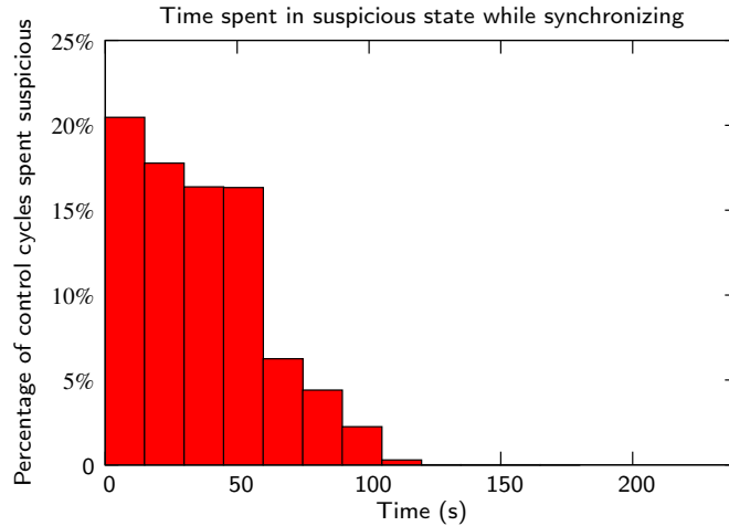
Figure 5.9: Average percentage of the control cycles spent in the suspicious state over intervals of 15 s during a run with 50 simulated robots in a 2.5 m × 2.5 m arena. The robots were not initially synchronized.
