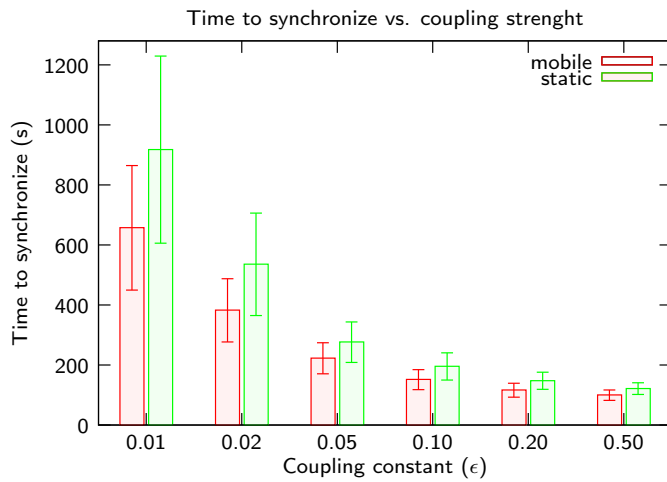
Figure 5.5: Synchronization rate a group of 50 simulated robots for coupling constants 0.01, 0.02, 0.05, 0.10, 0.20, 0.50. Each bar summarizes 100 runs and error-bars denote the standard deviation. The density was 6 robots/m 2 .
