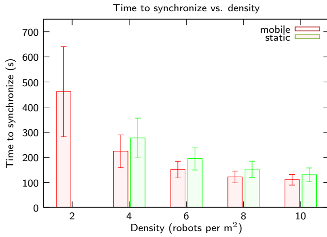
Figure 5.4: Synchronization rate in a group of 50 simulated robots at different densities. Each bar summarizes 100 runs and error-bars denote the standard deviation. A coupling constant of \epsilon = 0.1 was used in all runs. Due to the limited sensory range of the s-bots (up to 50 cm) experiments with static robots at a density of 2 robots/m 2 were not conducted. At this density, the interaction graph is almost never connected when the robots are distributed randomly.
