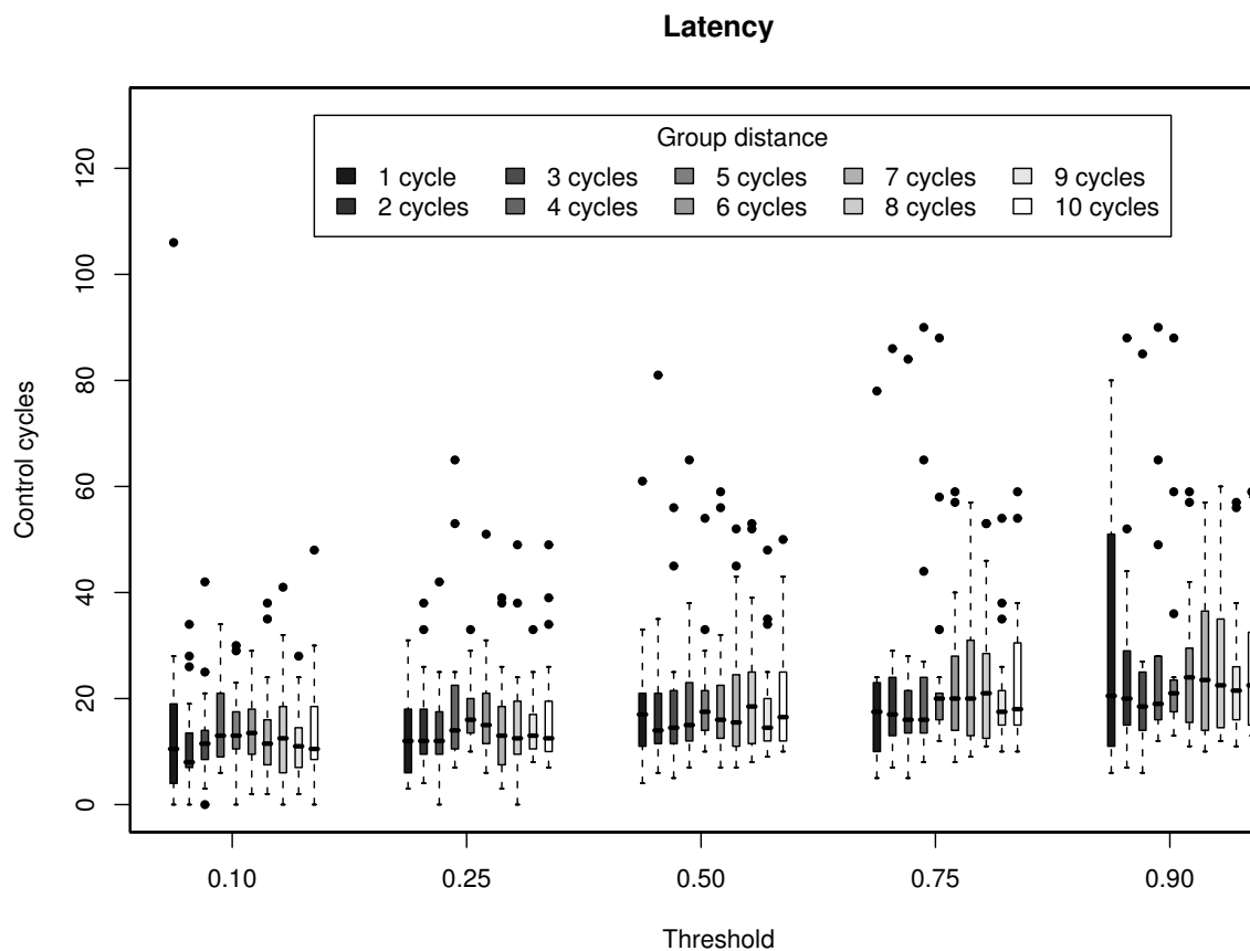
Figure 4.6: Box-plot of the latencies observed in 20 evaluation runs in the find_perimeter setup using fault detectors with input group distances from 1 to 10. Results are shown for the thresholds 0.10, 0.25, 0.50, 0.75, and 0.90. Each box comprises observations ranging from the first to the third quartile. The median is indicated by a horizontal bar, dividing the box into the upper and lower part. The whiskers extend to the farthest data points that are within 1.5 times the interquartile range. Outliers are shown as dots. The results show that the input group distance does not have a major influence on the latency of a fault detector, while larger thresholds yield longer latencies.
