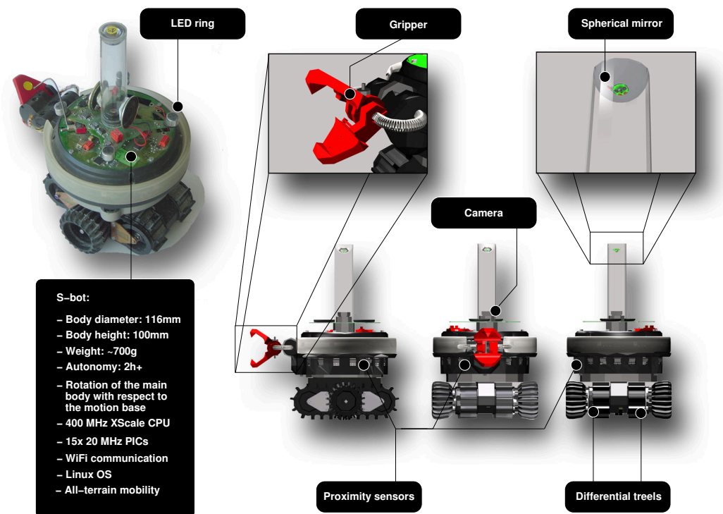
Figure 3.1: The s-bot : An autonomous, mobile robot capable of self-assembly. Processor: 400 MHz XScale CPU, operating system: Linux, weight: ~700 g, battery allows for ~2 h of operation between recharges.
