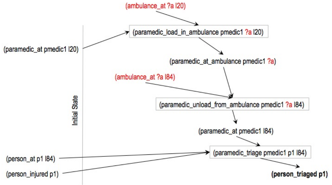
Figure 3.2: Partial solution plan developed by agent pmedic1
