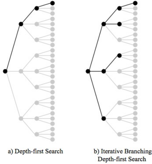
Figure 4.2: Comparison between the Depth-First Search algorithm and the Iterative Branching Depth-First Search algorithm with a hop count of 3, i.e. , when the algorithms have made 3 iterations.
