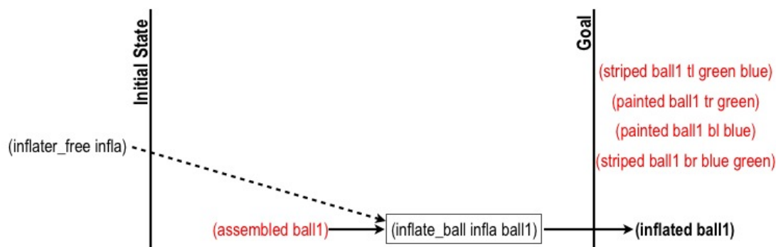
Figure 3.6: Partial solution plan developed by agent infla
