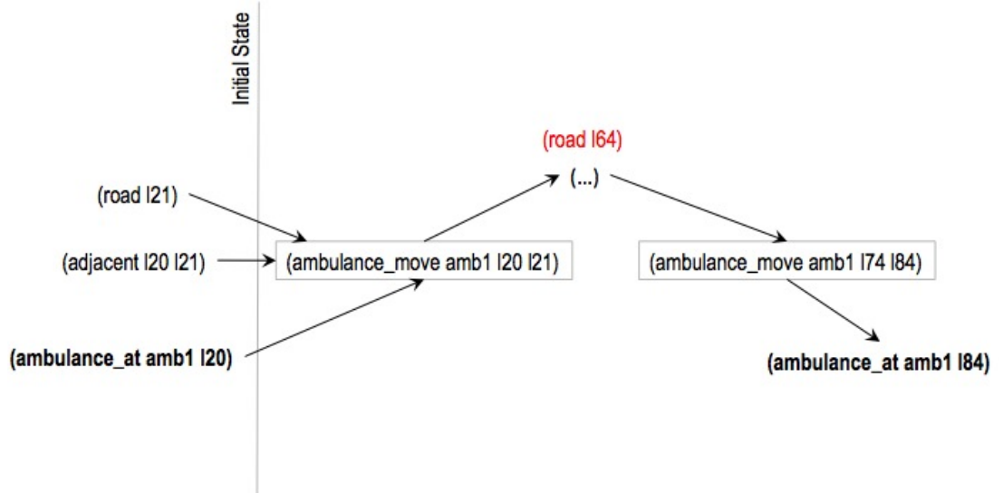
Figure 3.3: Partial solution plan developed by agent amb1
