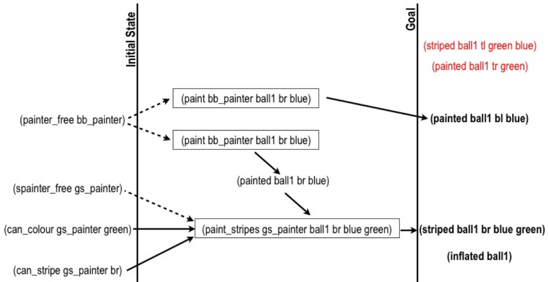
Figure 3.9: Partial solution plan developed by agent bbPainter
