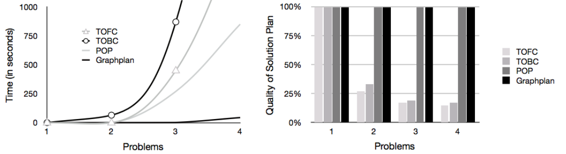
Figure 4.17: Results of the 3-block problems tests. On the left, evaluation of the performance of the planners. On the right, the quality of the solution plan relative to the optimal solution.
