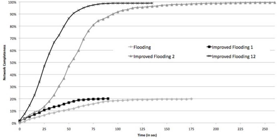
Figure 4.15: Comparison of different configurations of the Flooding algorithm
