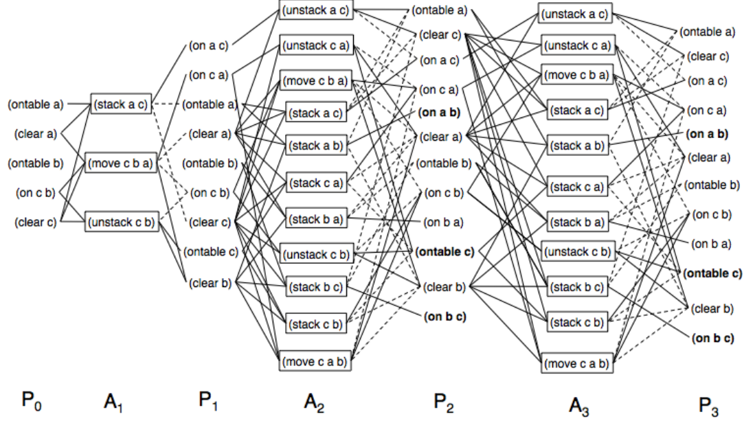
Figure 4.11: Agent stacker 's contribution in the Blocks World example problem.
