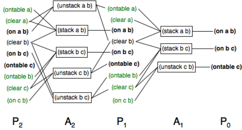
Figure 4.13: Agent unstacker 's contribution to the operators-graph in the Blocks World example problem.
