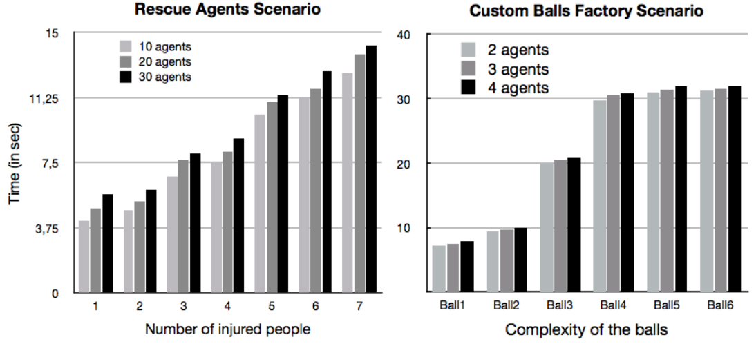
Figure 5.15: Evolution of performance of the Operators-graph-based Distributed Graphplan in both testing scenarios as skills distribution increase using a specific heuristic. The given number of agents is per skill.
