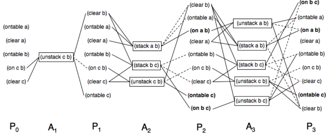
Figure 4.14: Planning graph generated by using the operators-graph in the Blocks World example problem.
