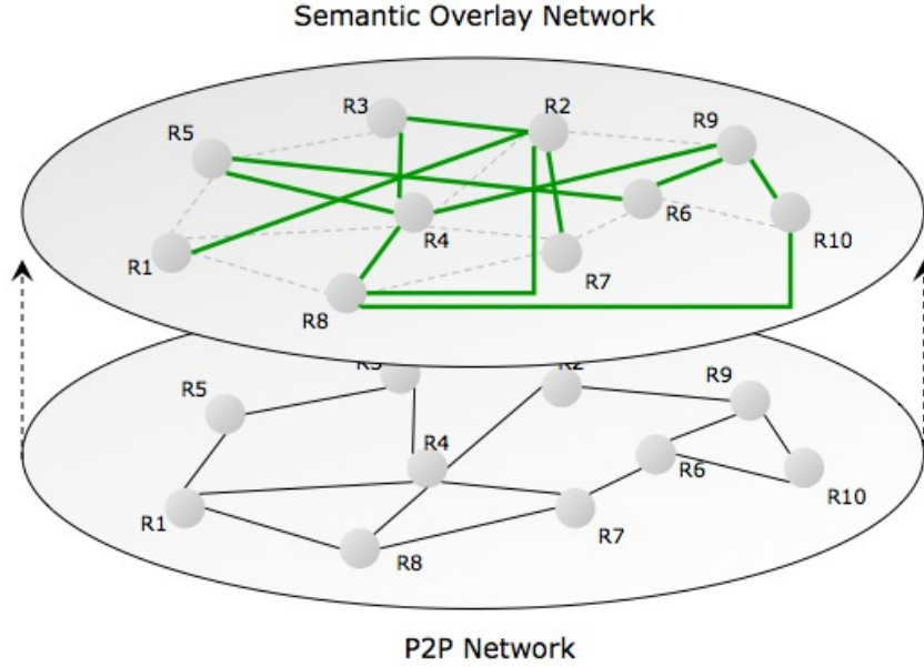
Figure 4.3: A semantic overlay network as a layer of the physical P2P network.
