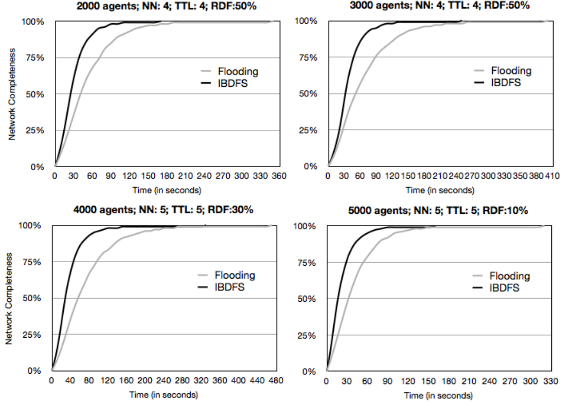
Figure 5.9: Comparison between the algorithms in larger networks
